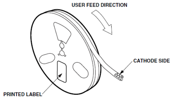
Figure 12: Reel Orientation
